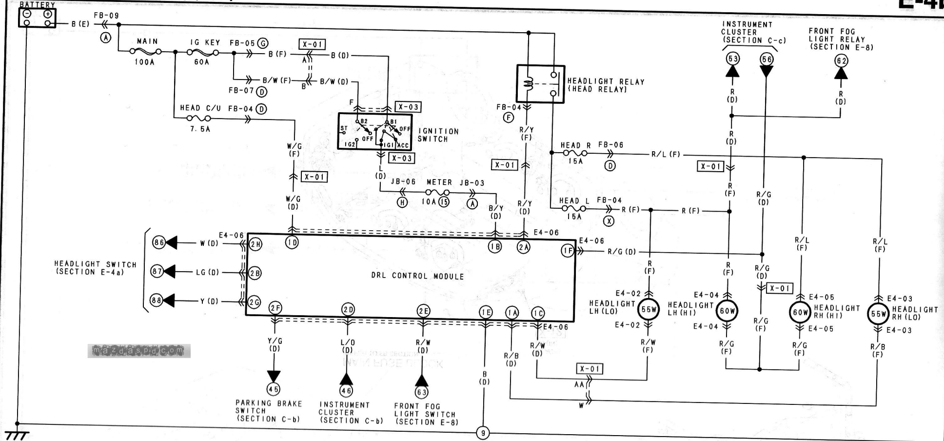
E4-02 HEADLIGHT LH (LO) (F)
